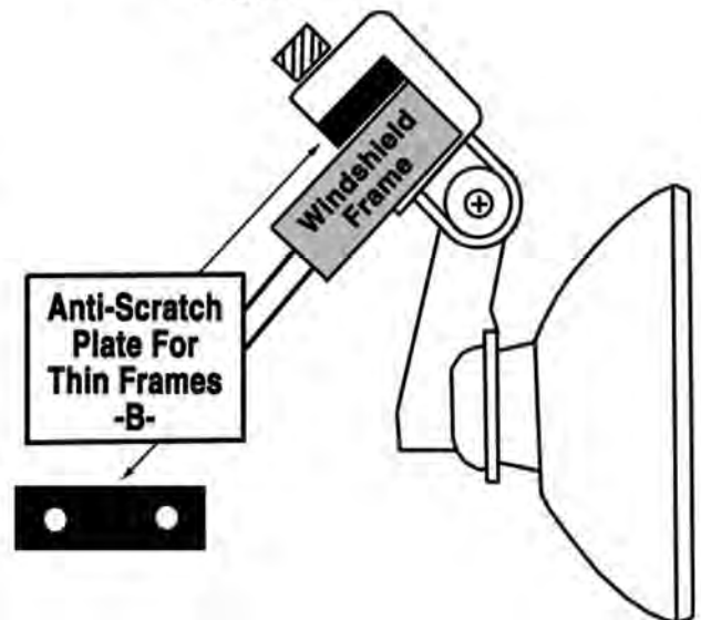
Mounted Below Windshield Fig. 2
